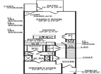
First Floor Plan Elevation A
