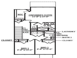
Second Floor Plan Elevation A
