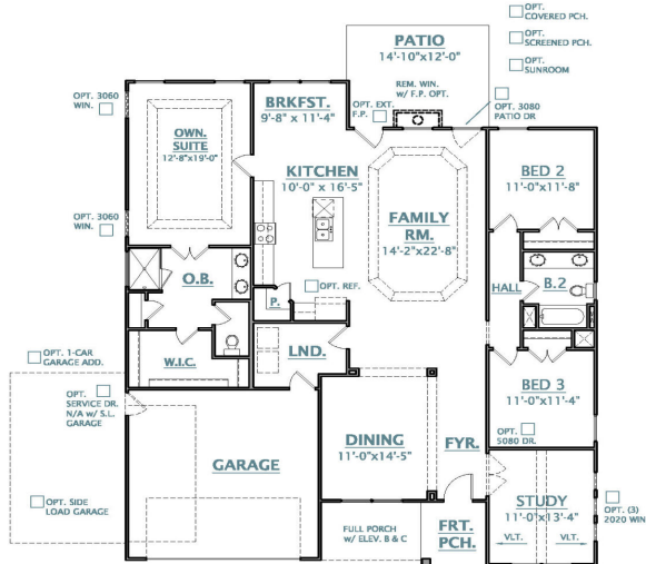
FLOOR PLAN
